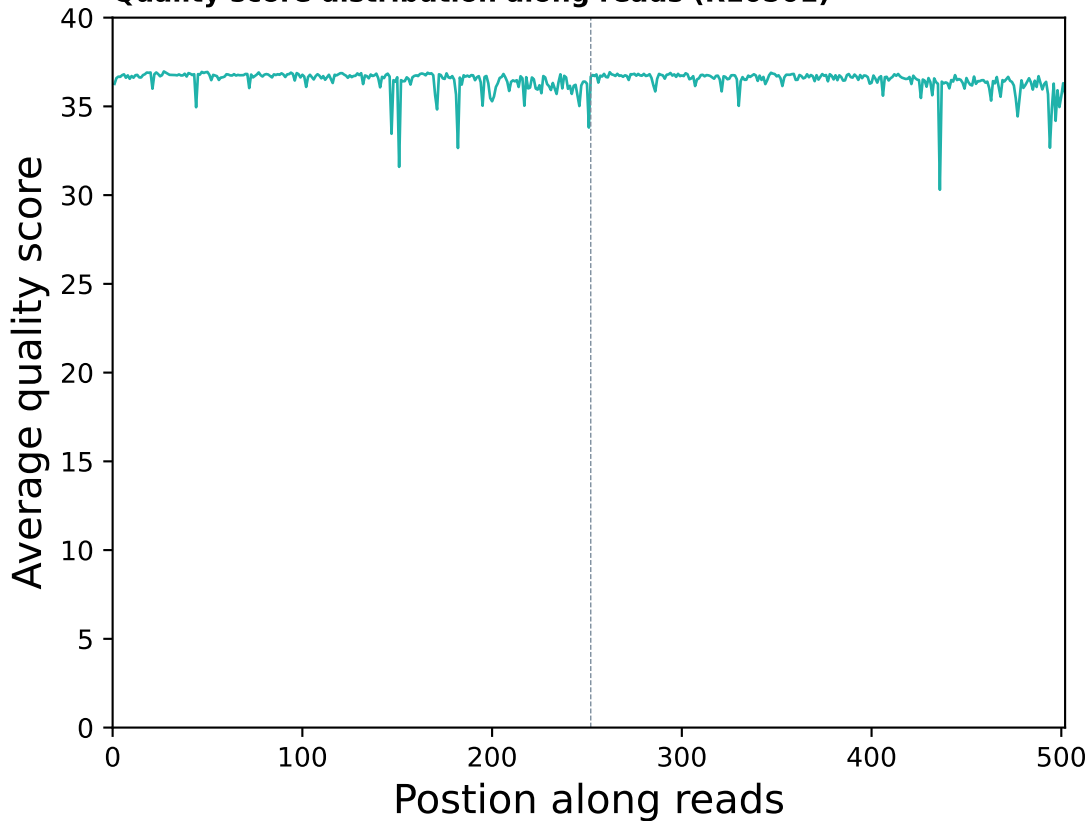
Quality score distribution along reads (R10501)
